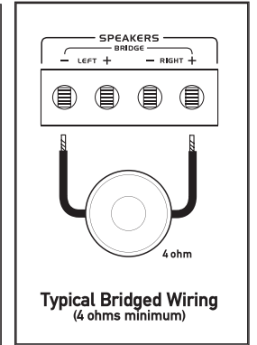
XPR522 speaker connections shown
