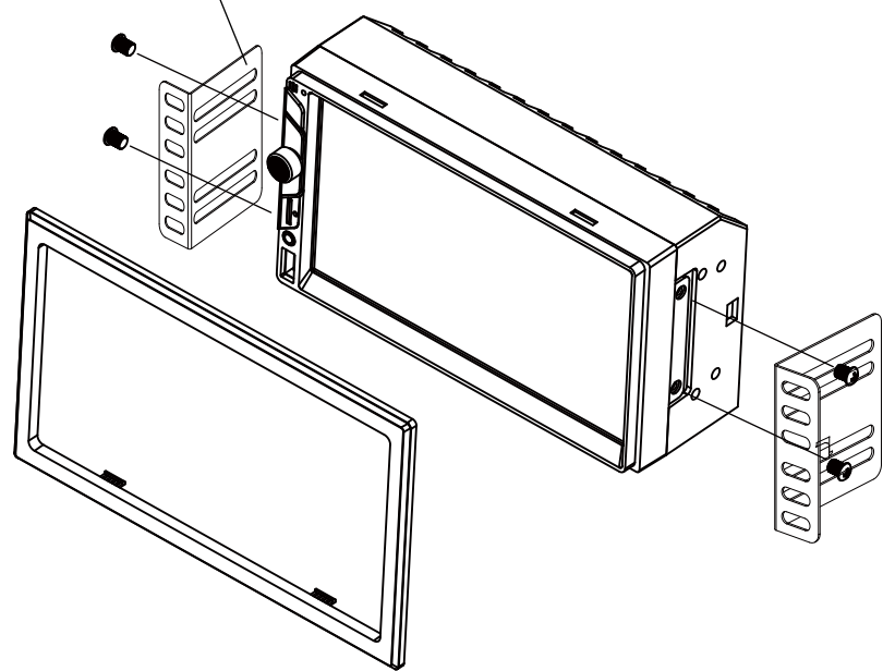
Typical Front-Load Mounting Method
